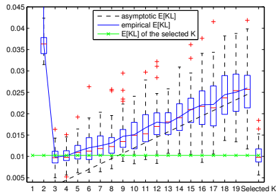
(c) Example MS with 2 000 data points
