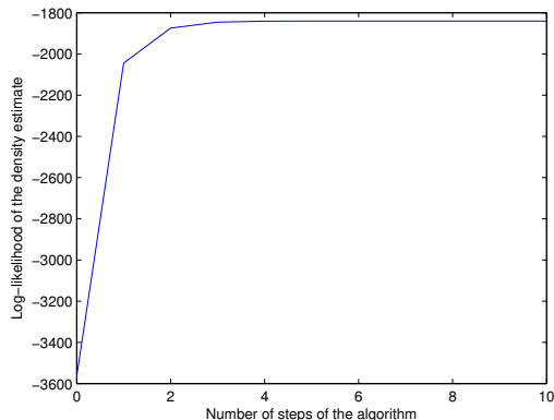
Figure 2: Increase of the Log-likelihood of the estimated density at each step of our iterative Newton-EM algorithm in the example NP with 3 components and 2 000 data points.
