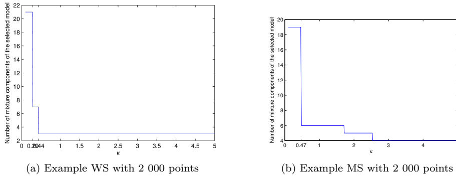
Figure 4: Slope heuristic: plot of the selected model dimension with respect to the penalty coefficient \kappa . In both examples, \hat{\kappa} is of order 1/2 .
