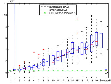
(b) Example WS with 10 000 data points
