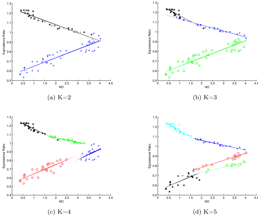
Figure 9: Clustering of NO data set into K classes. The strength of the color of the regression lines corresponds to the mixture proportion.
