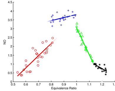
Figure 10: Clustering of NO data set into 4 classes, considering the regression of NO with respect to the equivalence ratio
