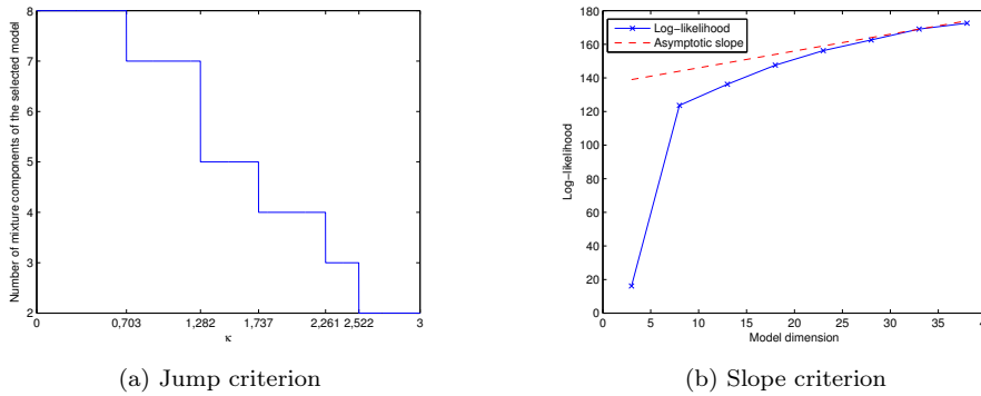
Figure 8: Slope heuristic for the ethanol data set
