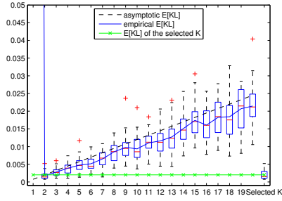
(a) Example WS with 2 000 data points
