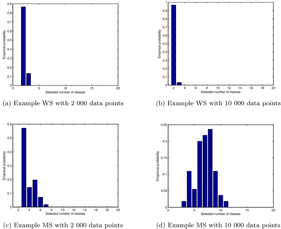
Figure 6: Histograms of the selected K
