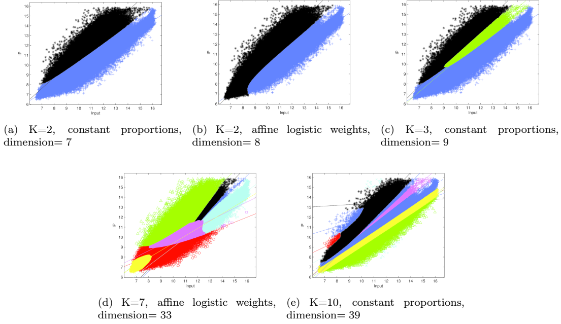
Figure 11: Clustering of ChIP-chip data set into K classes.
